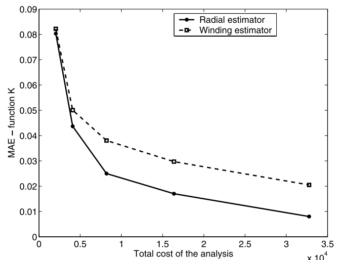
Fig. 7. Radial estimator vs winding stairs estimator for S_{\Pi} : best case – K function.
